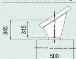
Particolare/Detail S
